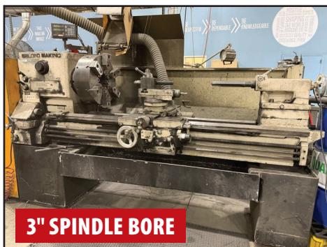
LEBLOND MAKINO REGAL SERVO SHIFT ENGINE LATHE
