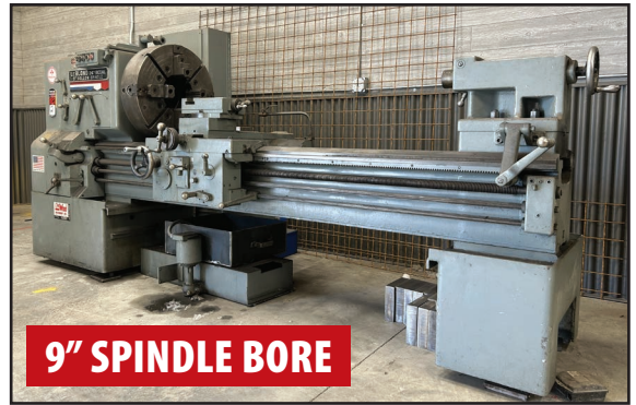
LEBLOND 24" X 80" REGAL HOLLOW SPINDLE LATHE
