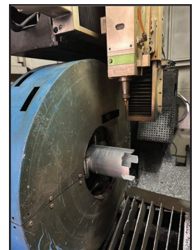
LASER HEAD
