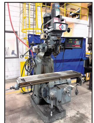
CLAUSING KONDIA VERTICAL MILL
