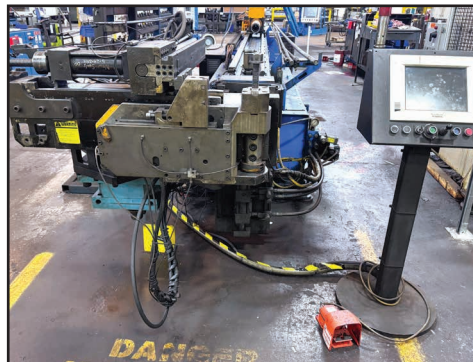
(2) EATON LEONARD VECTORBEND VB200 2" TUBE BENDERS
